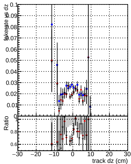
—•— DOM CKE TTbarPU —•— DOM mktFit TTbarPU-noDNN3 —•— DOM mktFit TTbarPU-clonerfix3
