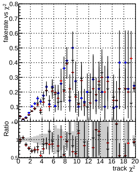
Fake rate vs. Legend: DOM CKF TTbarPU DOM CKF TTbarPU-noDNN3 BQM mktfit TTbarPU-clonerfix3
