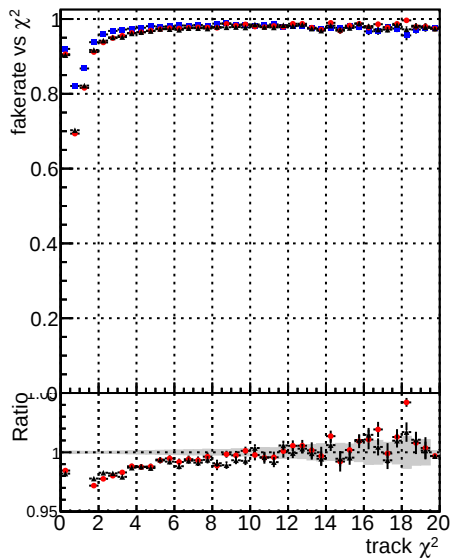
Fake rate vs. DOM CKF TTbarPU DOM mktFit TTbarPU-noDNN3 DOM mktFit TTbarPU-clonerfix3
