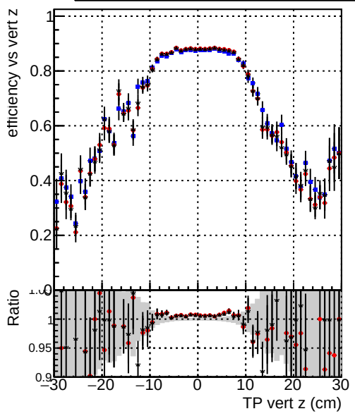
Efficiency vs. sim PV z — DQM_CKF_TTbarPU — DQM_mkFit_TTbarPU-noDNN3 — DQM_mkFit_TTbarPU-clonerfix3
