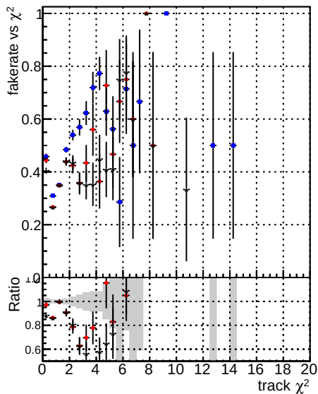
Fake rate vs. DOM CKF TTbarPU DOM CKF TTbarPU-noDNN3 DOM CKF TTbarPU-clonerfix3
