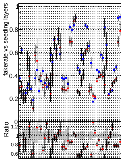
Fake rate vs. DOM CKF TTbarPU DOM CKF TTbarPU-noDNN3 DOM CKF TTbarPU-clonerfix3
