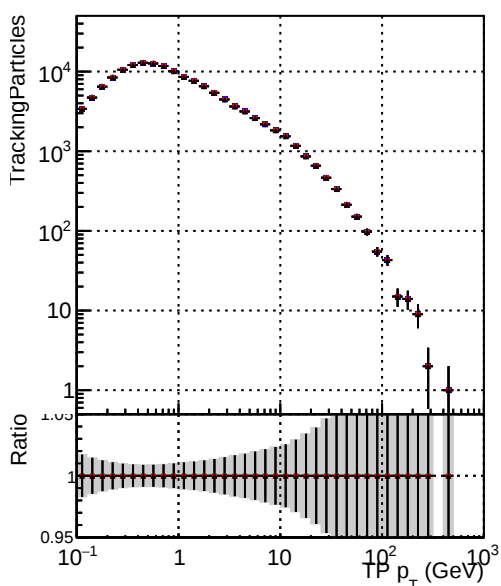
● DQM_CKF_TTbarPU + DQM_mkFit_TTbarPU-noDNN3 + DQM_mkFit_TTbarPU-clonerfix3
