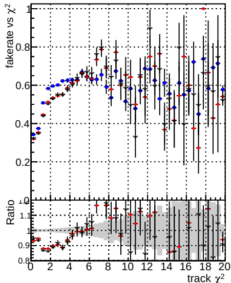
Fake rate vs. — DOM CKE TTbarPU — DOM mktFit TTbarPU-noDNN3 — DOM mktFit TTbarPU-clonerfix3
