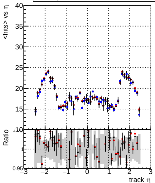
mean hit — DQM_CKF_TTbarPU — DQM_mkFit_TTbarPU — DQM_mkFit_TTbarPU-clonerfix2
