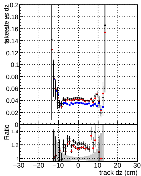
Fake rate vs dz — DOM CKF TTbarPU — BOM mktFit TTbarPU-clonerfix2
