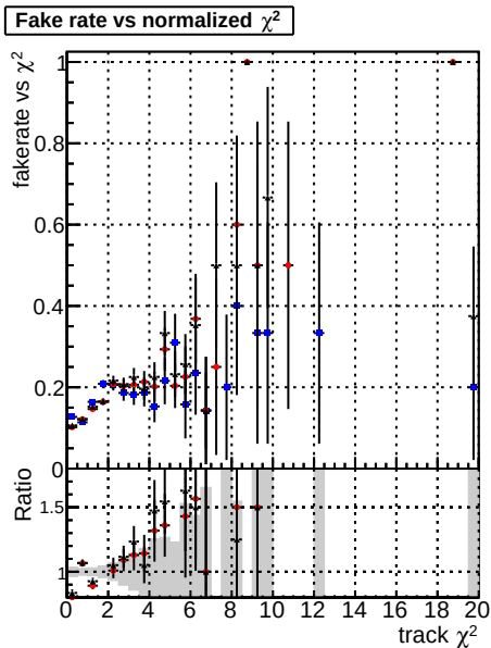
Fake rate vs. DOM CKF TTbarPU BQM mkttt TTbarPU-clonerfix2
