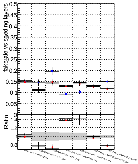
Fake rate vs. DOM CKF TTbarPU BQM mkttt TTbarPU-clonerfix2
