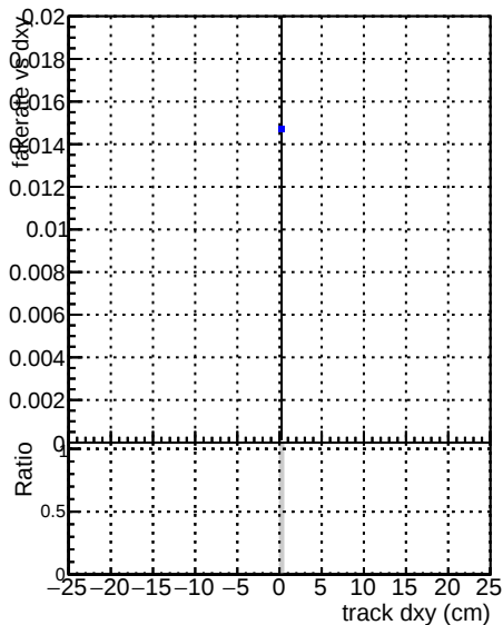
Legend for Fake rate vs dxy and Fake rate vs dz: DOM CKF TTbarPU (Blue dot) DOM mktFit TTbarPU-clonerfix2 (Red dot)
