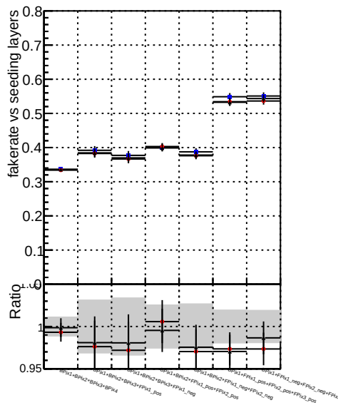
Fake rate vs. Legend: DOM, CKF, TTbarPU, BQM, mkt, TTbarPU-clonerfix2
