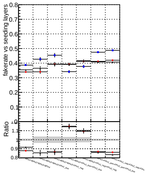
Fake rate vs. DOM CKE TTbarPU DOM mkttt TTbarPU-clonerfix2
