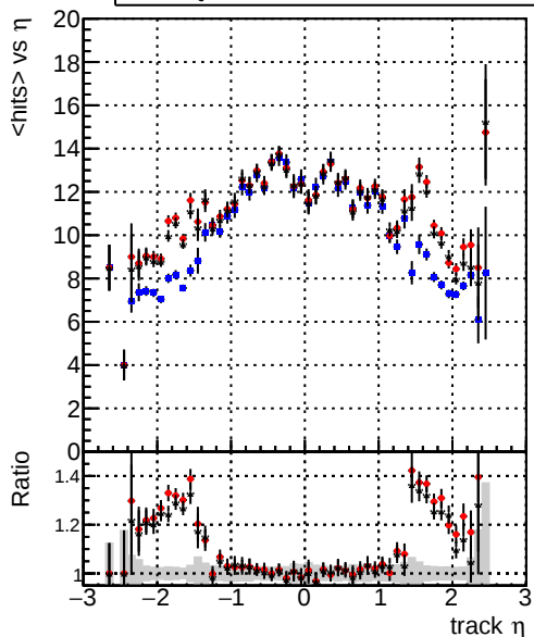
mean hit — DQM_CKF_TTbarPU — DQM_mkFit_TTbarPU — DQM_mkFit_TTbarPU-clonerfix2
