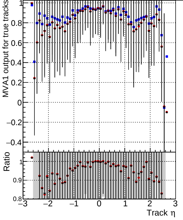
MVA1 of associated tracks (recoToSim) vs. track \eta Legend: DQM_CKF_TTbarPU (blue squares) DQM_mkFit_TTbarPU (red circles) DQM_mkFit_TTbarPU-clonerfix2 (black triangles)
