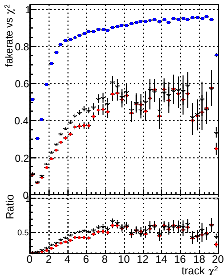
Legend: DOM (blue circles), CKF (black crosses), TTbarPU (red crosses), BOM (grey crosses). Fake rate vs. BOM mktfit TTbarPU-clonerfix2
