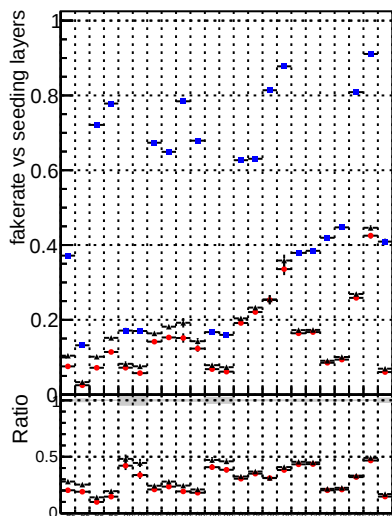
Legend: DOM (blue circles), CKF (black crosses), TTbarPU (red crosses), BOM (grey crosses). Fake rate vs. BOM mktfit TTbarPU-clonerfix2
