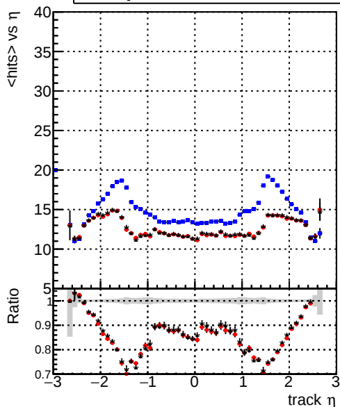
mean hit — DQM_CKF_TTbarPU — DQM_mkFit_TTbarPU — DQM_mkFit_TTbarPU-clonerfix2
