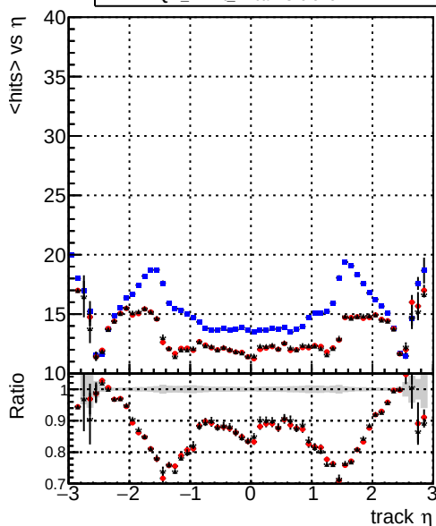
mean hits vs \eta — DQM_CKF_TTbarPU — DQM_mkFit_TTbarPU — DQM_mkFit_TTbarPU-clonerfix2
