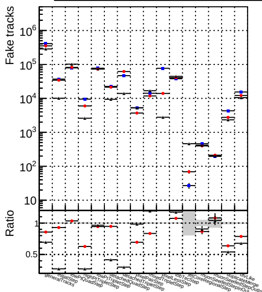
Number Legend —●— DQM_mkFit_TTbarPU —★— DQM_mkFit_TTbarPU-clonerfix
