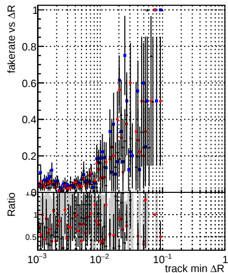
Legend: DQM_CKF_TTbarPU (blue circles) DQM_mkFit_TTbarPU (red circles) DQM_mkFit_TTbarPU-clonerfix (black circles with error bars)
