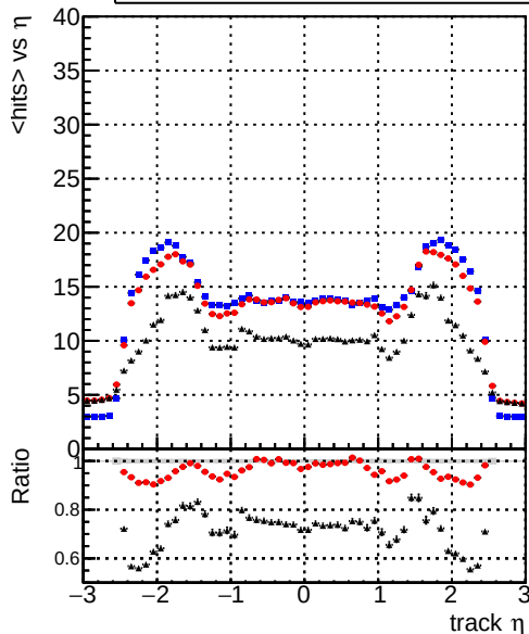
— DQM_CKF_TTbarPU — DQM_mkFit_TTbarPU — DQM_mkFit_TTbarPU-clonerfix mean hits
