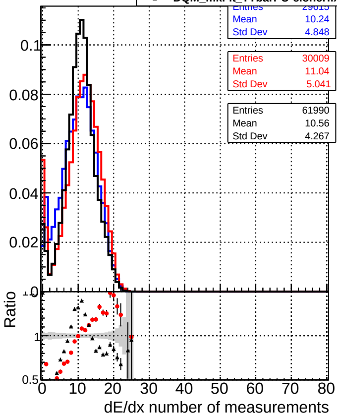
—■— DQM_CKF_TTbarPU —●— DQM_mkFit_TTbarPU —▲— DQM_mkFit_TTbarPU-clonerfix
