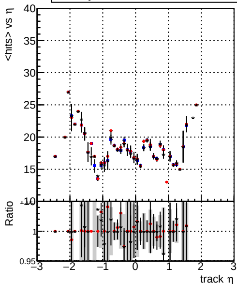
mean hits — DQM_CKF_TTbarPU — DQM_mkFit_TTbarPU — DQM_mkFit_TTbarPU-clonerfix
