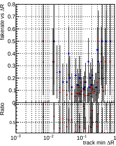
Fake rate vs \Delta R(\text{track, jet}) Legend: DOM_CKF_TTbarPU (blue dots) DOM_mkFit_TTbarPU (red dots) DOM_mkFit_TTbarPU-clonerfix (black dots)
