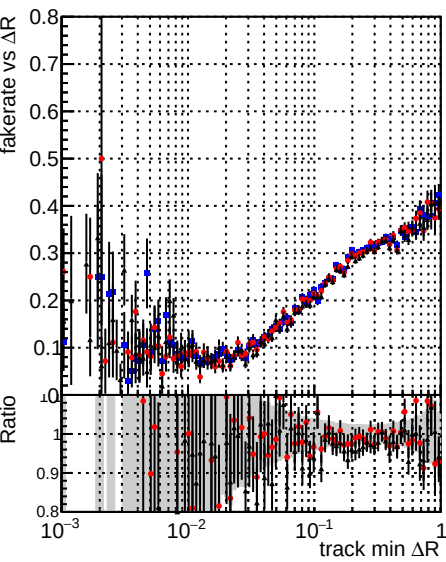
Fake rate vs \Delta R(\text{track, jet}) DQM_CKF_TTbarPU DQM_mkFit_TTbarPU DQM_mkFit_TTbarPU-clonerfix
