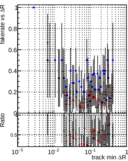
Legend: DQM_CKF_TTbarPU (blue dots), DQM_mkFit_TTbarPU (red dots), DQM_mkFit_TTbarPU-clonerfix (black dots with error bars)
