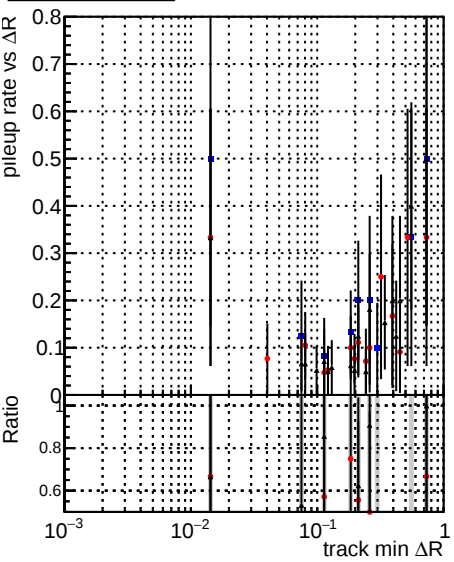
Legend: DQM_CKF_TTbarPU (blue dots), DQM_mkFit_TTbarPU (red dots), DQM_mkFit_TTbarPU-clonerfix (black dots with error bars)
