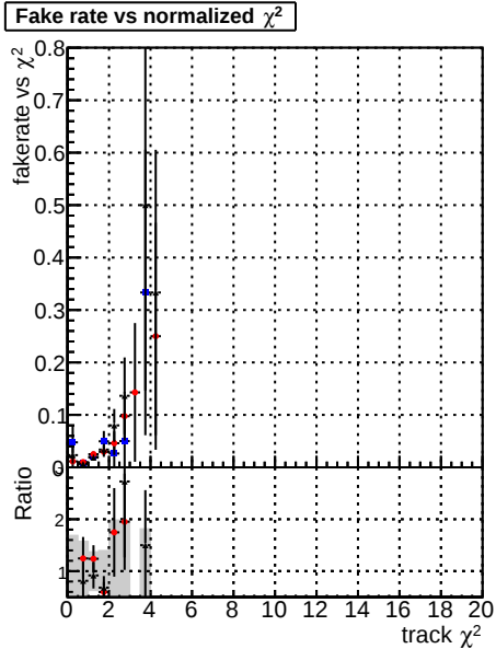
Fake rate vs. \chi^2 Legend: DOM (blue), CKF (red), TTbarPU (black), DOM mktfit (grey), TTbarPU-clonerfix (grey)
