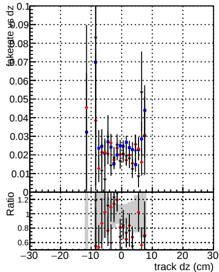
Fake rate vs dz —●— DOM CKF TTbarPU —●— BQM mktFit TTbarPU-clonerfix
