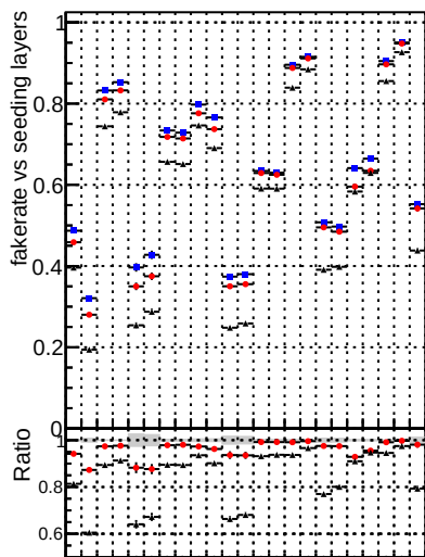
Fake rate vs. DOM CKF TTbarPU BQM mktfit TTbarPU-clonerfix
