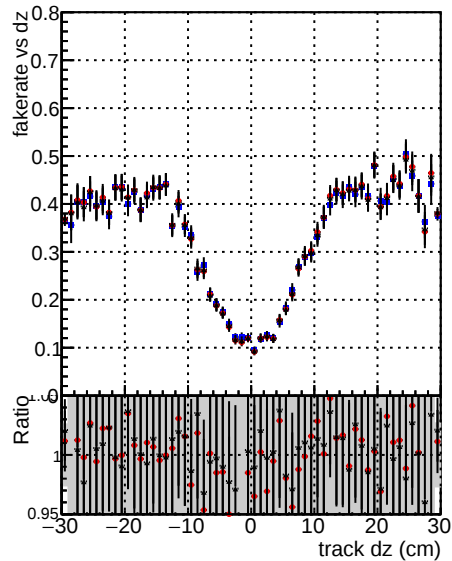
DOM CKE SoftQCD DOM mktFit SoftQCD DOM mktFit SoftQCD-fixCloner
