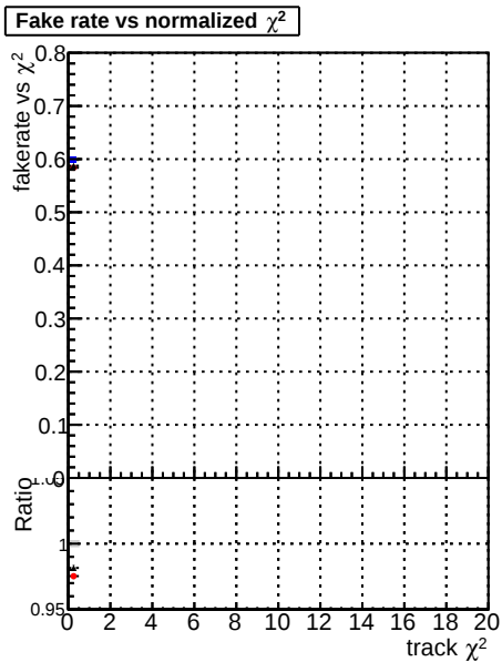
Fake rate vs. Legend: DOM CKF SoftQCD DOM mktFit SoftQCD-fixCloner
