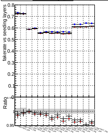
Fake rate vs. Legend: DOM CKF SoftQCD DOM mktFit SoftQCD-fixCloner
