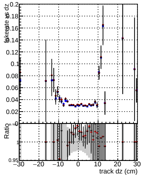
— DOM CKE SoftQCD — DOM mkFit SoftQCD — DOM CKE SoftQCD-fix — DOM mkFit SoftQCD-fixCloner
