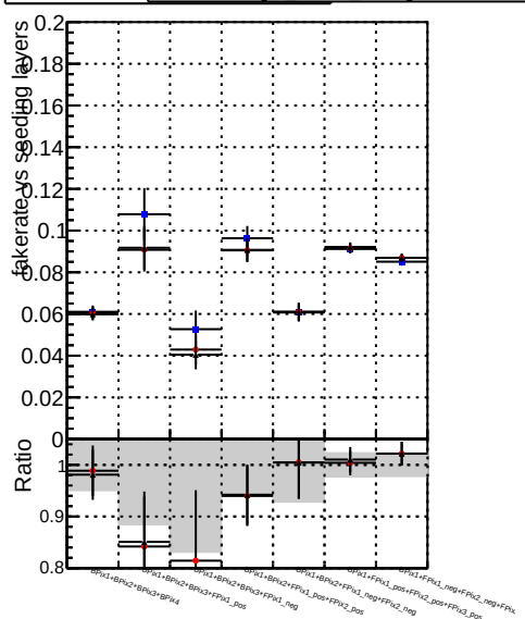
Fake rate vs. DOM CKF SoftOCD DOM mktFit SoftOCD-fix DOM mktFit SoftCloner
