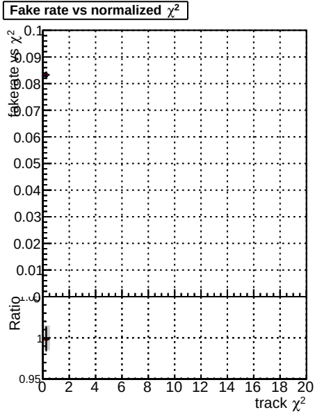
Fake rate vs. DOM CKF SoftOCD DOM mktFit SoftOCD-fix DOM mktFit SoftCloner
