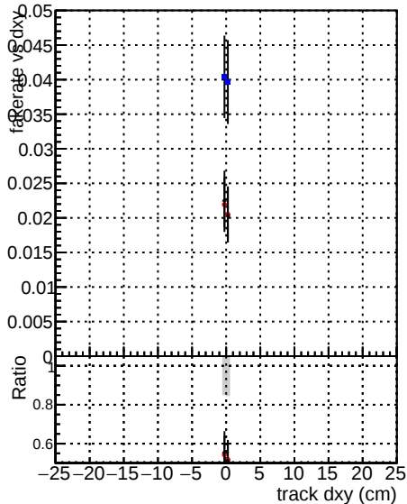
— DOM CKF SoftQCD — BOM mktFit SoftQCD-fixCloner
