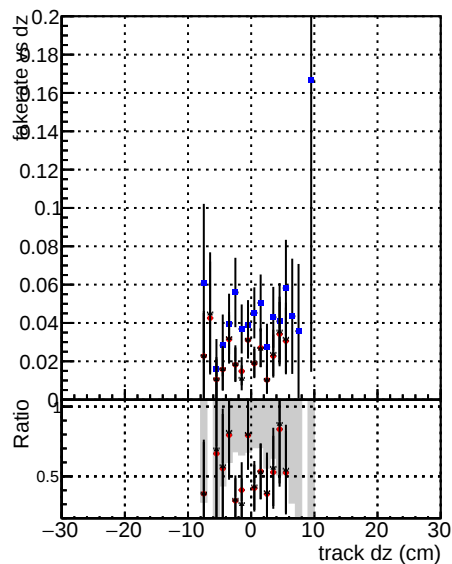
— DOM CKF SoftQCD — BOM mktFit SoftQCD-fixCloner
