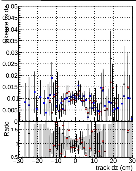
Fake rate vs dz DOM CKE SoftQCD DOM mktFit SoftQCD-fixCloner
