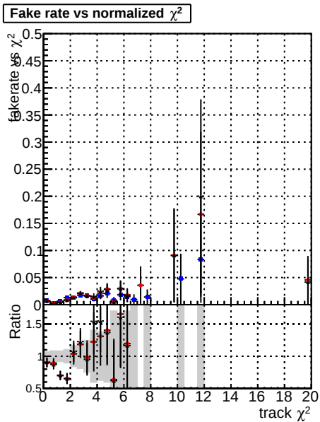
Fake rate vs. Legend: DOM (blue), CKF (red), SoftOCB (green), BQM (black), BQM-mkFit (purple), SoftOCB-fix (orange), Cloner (pink)
