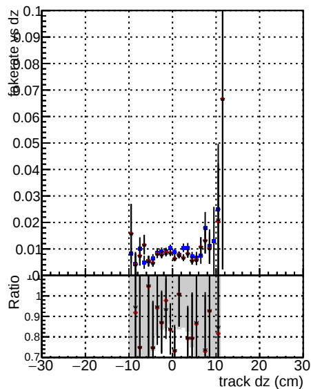
— DOM CKF SoftQCD — DOM CKF SoftQCD-fixCloner — DOM mktFit SoftQCD-fixCloner
