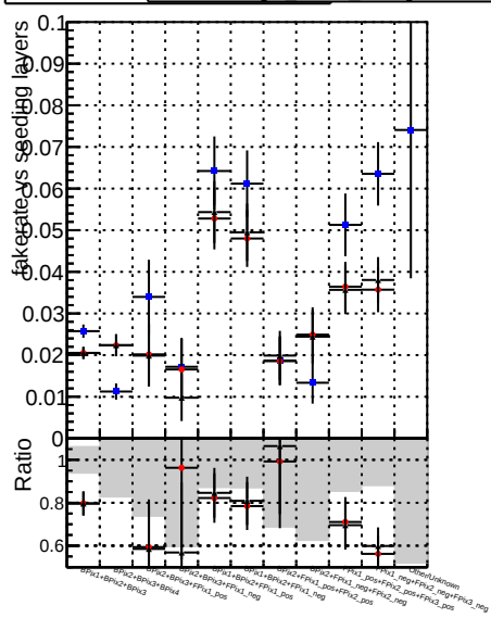
Fake rate vs. Legend: DOM, CKF, SoftQCD, SoftQCD-fix, Cloner
