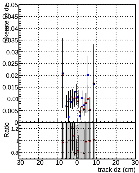
— DOM CKF SoftQCD — DOM CKF SoftQCD-fixCloner — DOM mktFit SoftQCD
