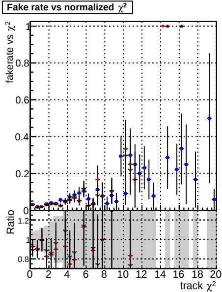
Fake rate vs. DOM CKF SoftQCD DOM CKF SoftQCD-fix
