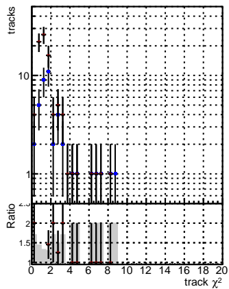
N of reco track vs. \chi^2 DQM Ckf 3-merged DQM Ckf 3-merged DQM mkFit SoftQCD-fixCloner
