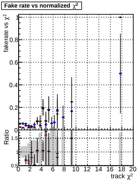
Fake rate vs. \chi^2 Legend: DOM, CKF, SoftOCB, SoftOCB-fixCloner
