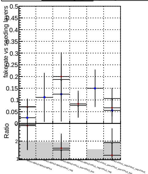
Fake rate vs. DOM CKF SoftQCD DOM mktFit SoftQCD-fix Cloner
