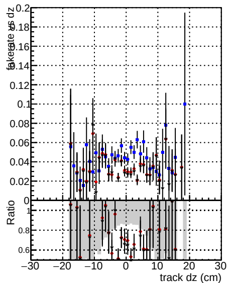
Fake rate vs dz DOM CKF SoftQCD DOM CKF SoftQCD-fixCloner
