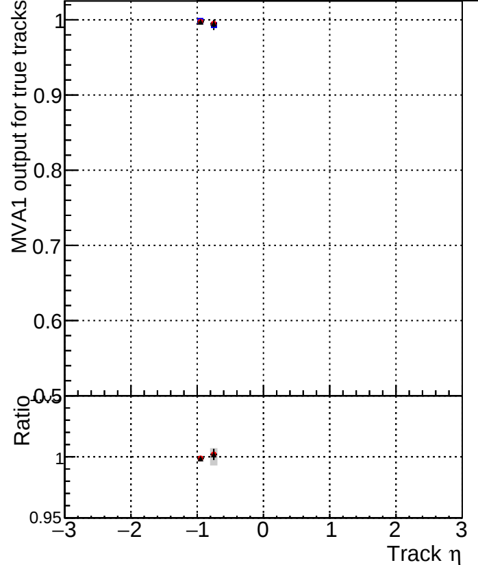
MVA1 of associated tracks (recoToSim) vs. track \eta Legend: DQM_CKF_SoftQCD (blue squares) DQM_mkFit_SoftQCD- (red circles) DQM_mkFit_SoftQCD-fixCloner (black triangles)
