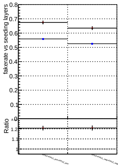
Fake rate vs. Legend: DOM CKF TTbar (blue), DOM mkt TTbar (red), DOM mkt TTbar-newTr2 (black)
