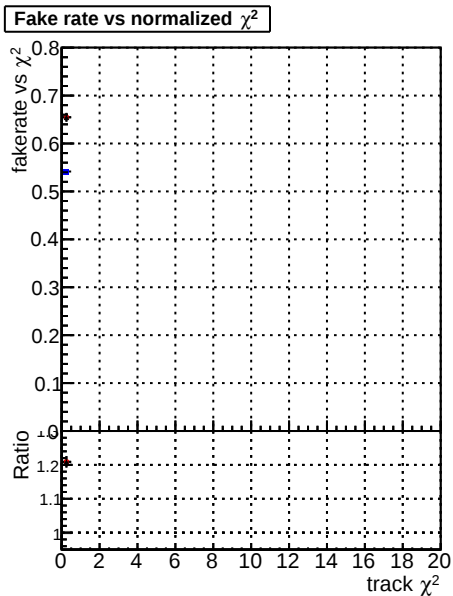
Fake rate vs. Legend: DOM CKF TTbar (blue), DOM mkt TTbar (red), DOM mkt TTbar-newTr2 (black)
