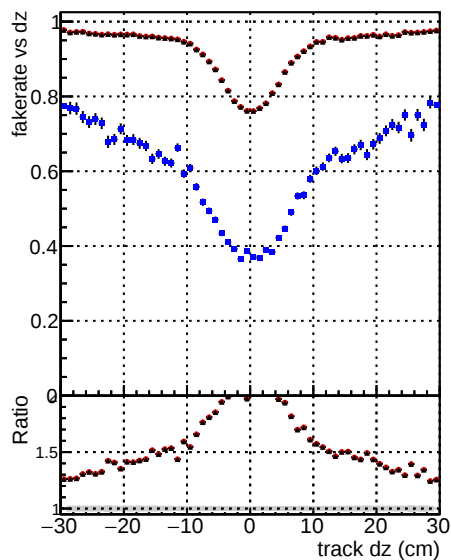
DOM CKF T\bar{T} bar DOM mkt T\bar{T} bar DOM mkt T\bar{T} bar-newTr2
