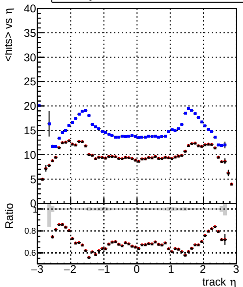
mean hits — DQM_CKF_TTbar — DQM_mkFit_TTbar — DQM_mkFit_TTbar-newTr2
