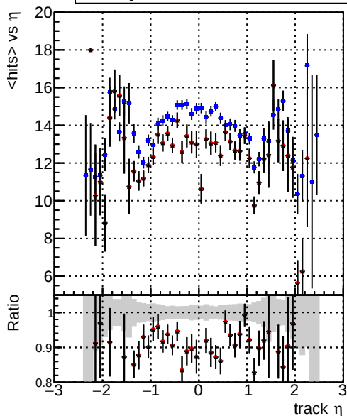
— DQM_CKF_TTbar — DQM_mkFit_TTbar — DQM_mkFit_TTbar-newTr2 mean hit
