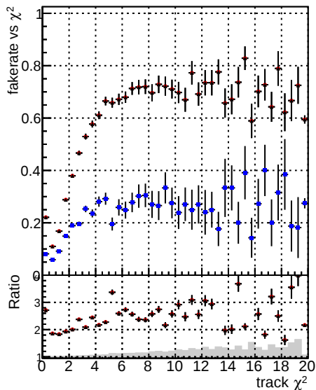
Fake rate vs. DOM CKF TTbar DOM mktFit TTbar DOM mktFit TTbar-newTr2
